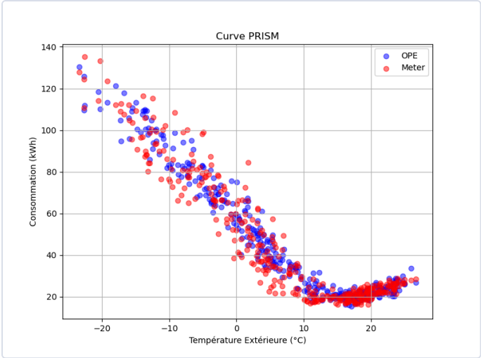
Figure — Courbe PRISM · Model vs. measured data
